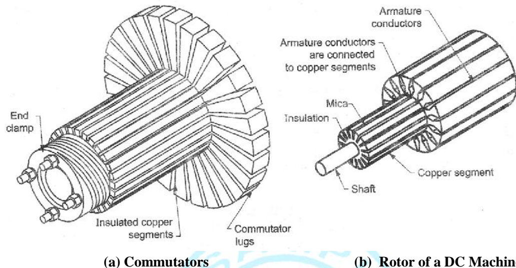
Figure-7 : Construction of a Commutator
