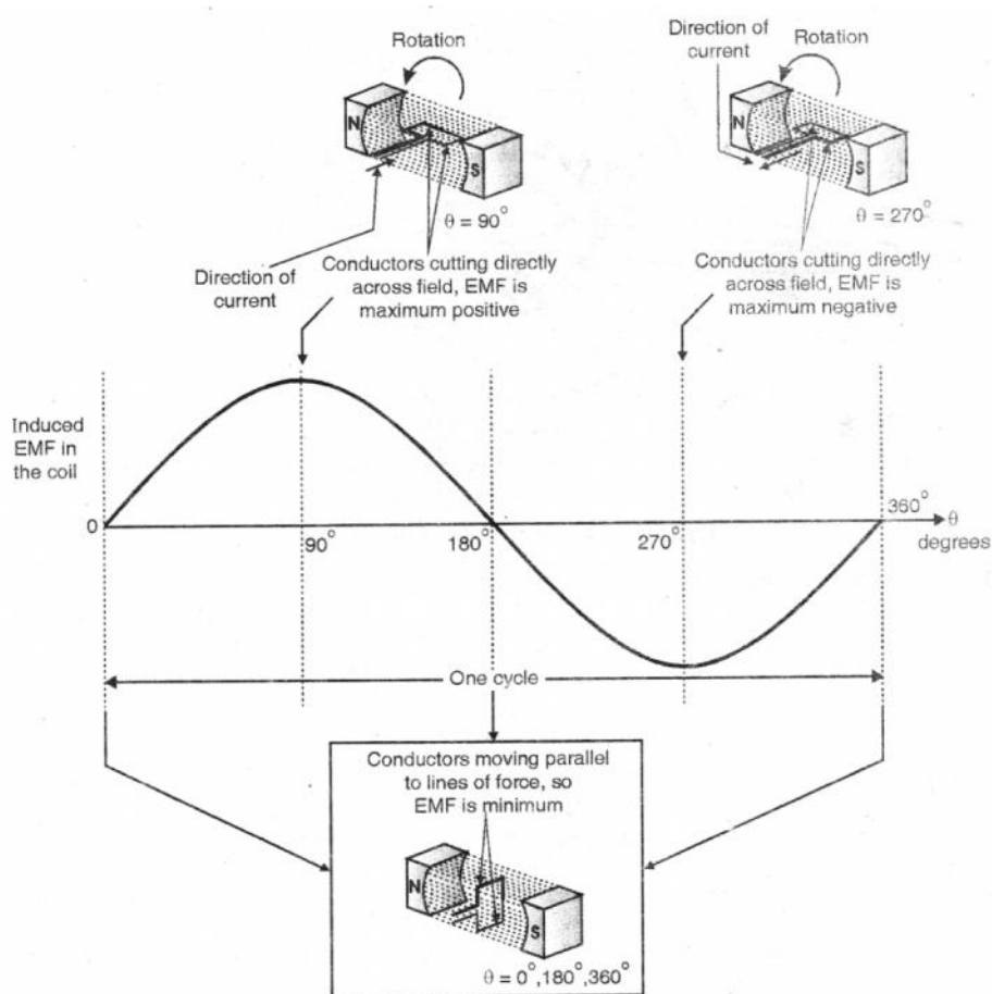
Figure-5: Shape of induced emf and corresponding positions of single turn coil
