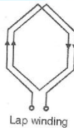
Figure-8(a) : Simplified diagram of Lap winding
