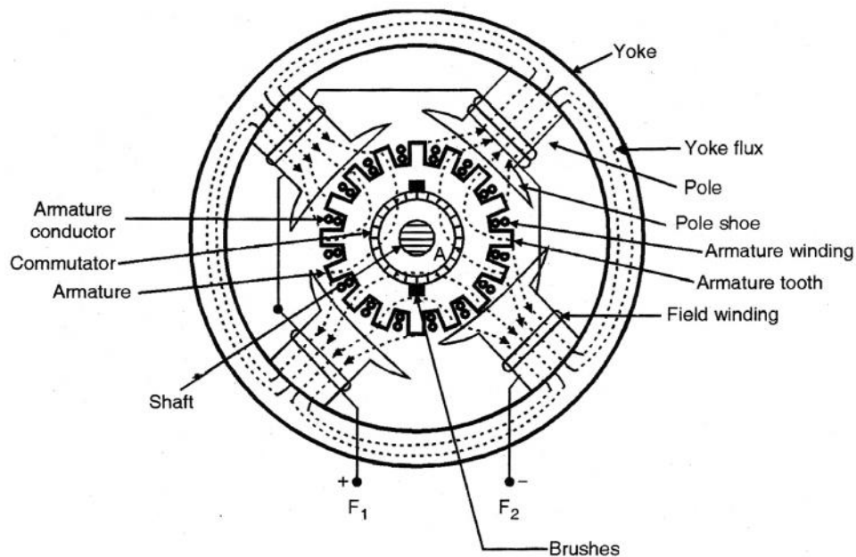
Figure-6 : Construction of a dc generator
