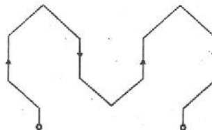
Figure-8(b): Simplified diagram of wave winding
